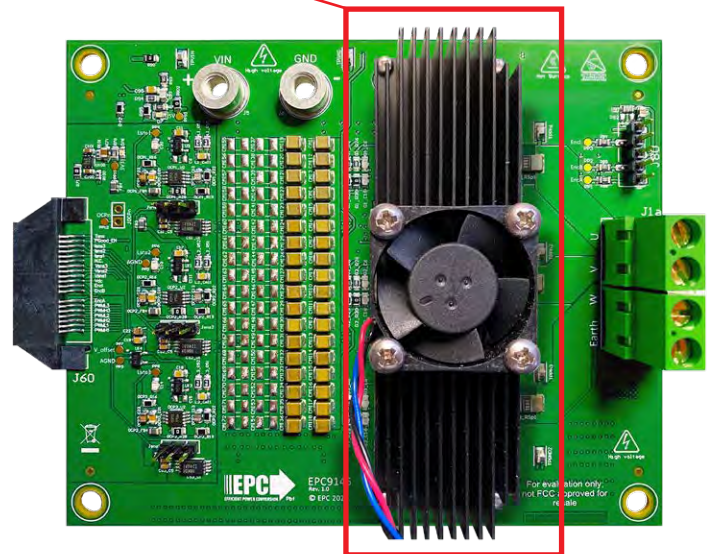
Forced Air Cooling
