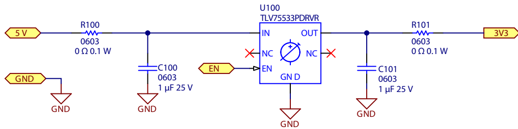
Figure 18: 5 V to 3.3 V LDO power supply
