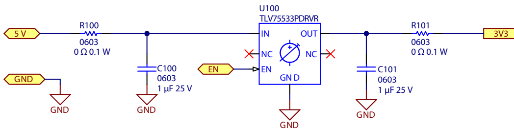
Figure 25: 5 V to 3.3 V LDO power supply schematic
