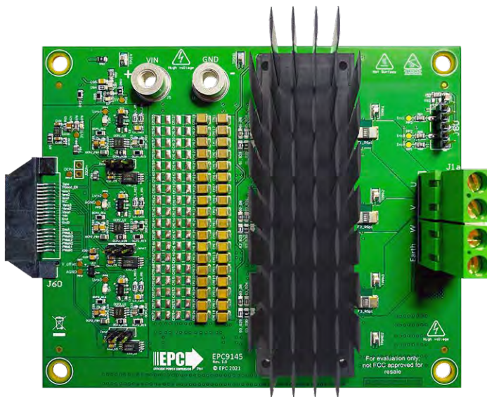
Natural Convection Cooling
