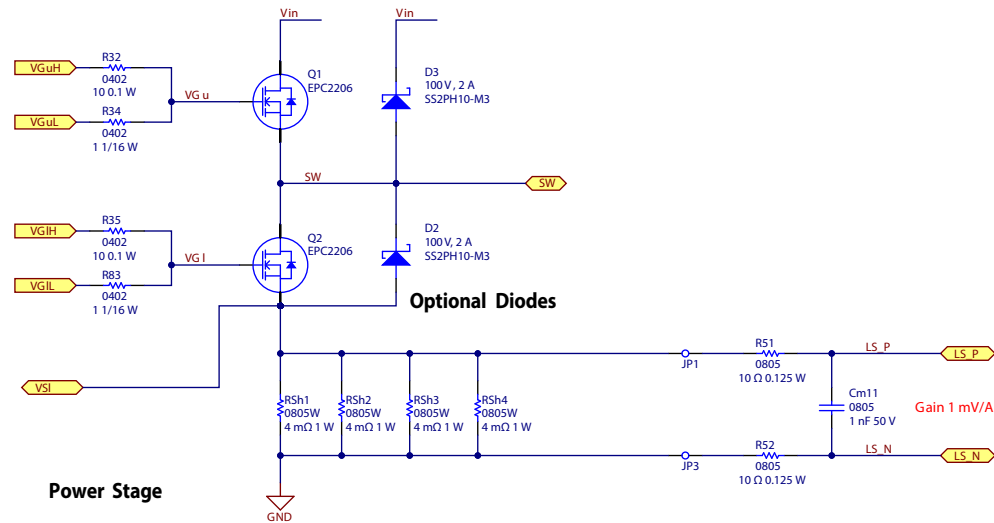
Figure 17: EPC2206 Phase-Leg
