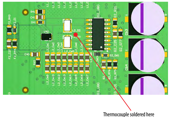
Figure 13: Thermocouple location on the bottom side of the PCB
