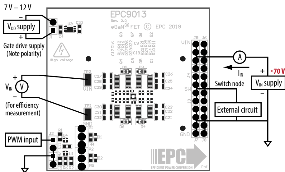
Figure 2: Proper connection and measurement setup
