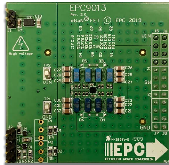
EPC9013 development board
