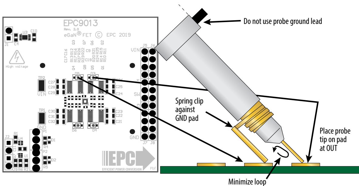
Figure 3: Proper Measurement of Switch Node – V_{SW}
