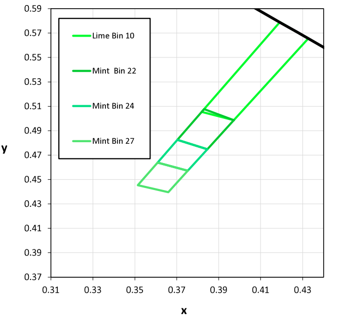
Figure 8. Color bin structure for LUXEON C Mint and Lime for Table 7.
