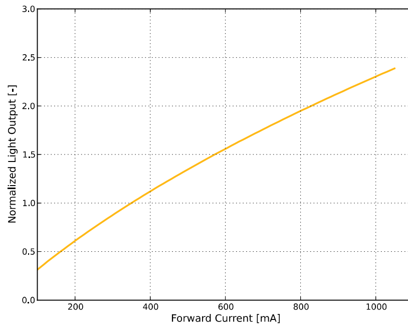
Figure 3c. Typical normalized light output vs. forward current for LUXEON C PC Amber at T_j=85^{\circ}\text{C} .
