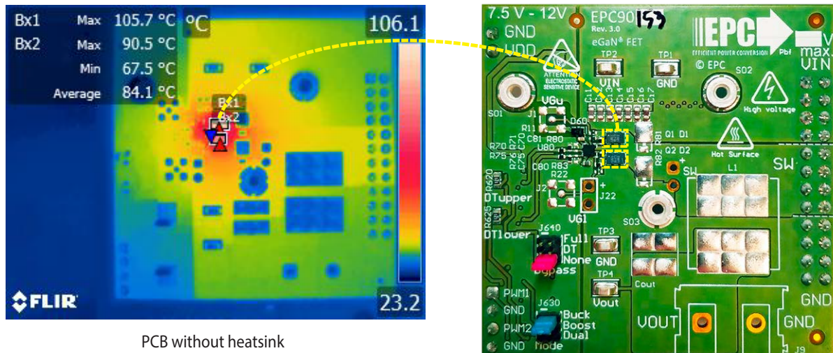
Figure 16: Measured thermal image readings of case temperature when operating under the following conditions: f_s = 500 \text{ kHz} , I_{OUT} = 28 \text{ A} output, 25^\circ\text{C} ambient and high air flow
