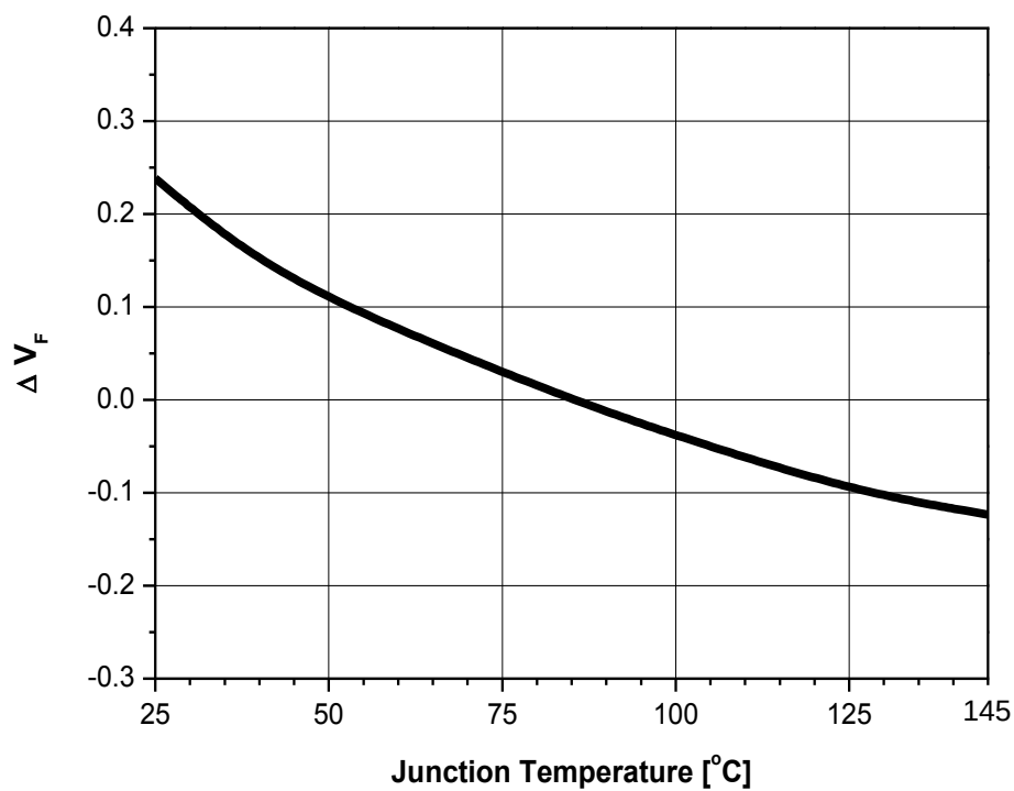
Fig 8b. Relative Forward Voltage vs. Junction Temperature for Y11-XX-XX-B, I_F=175\text{mA}
