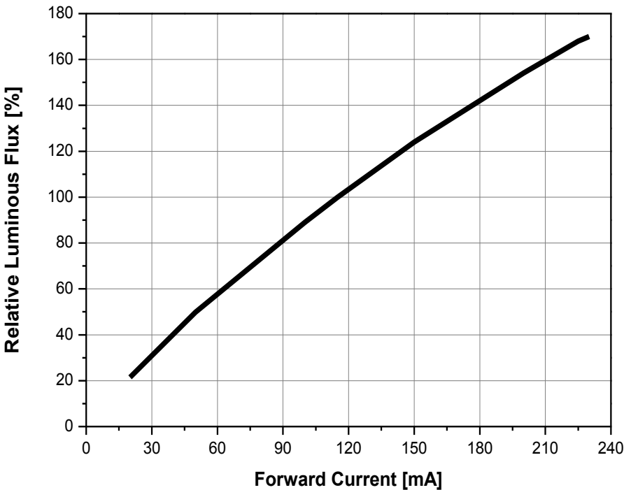
Fig 4c. Forward Current vs. Relative Luminous Flux for Y11-XX-XX-C, T_j=85^{\circ}\text{C}
