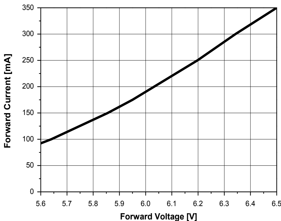
Fig 3b. Forward Voltage vs. Forward Current for Y11-XX-XX-B, T_j=85^{\circ}\text{C}
