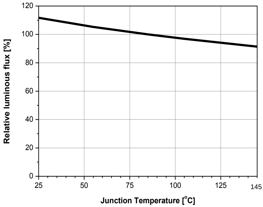
Fig 7c. Relative Light Output vs. Junction Temperature for Y11-XX-XX-C, I_F=115\text{mA}
