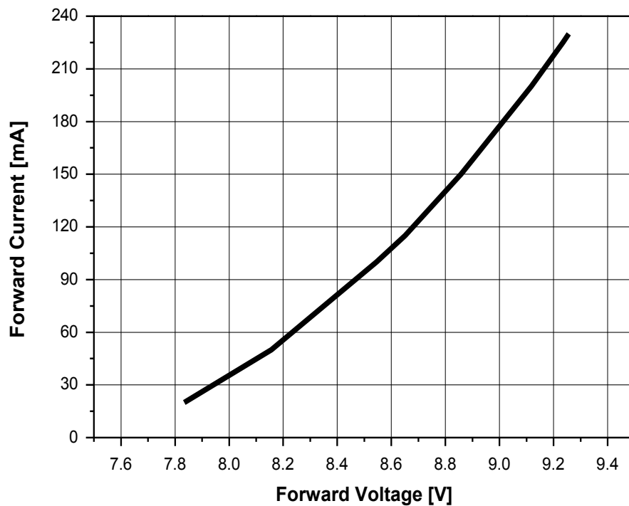
Fig 3c. Forward Voltage vs. Forward Current for Y11-XX-XX-C, T_j=85^{\circ}\text{C}
