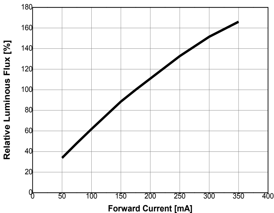
Fig 4b. Forward Current vs. Relative Luminous Flux for Y11-XX-XX-B, T_j=85^{\circ}\text{C}
