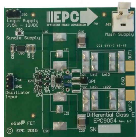
EPC9054 amplifier board photo
