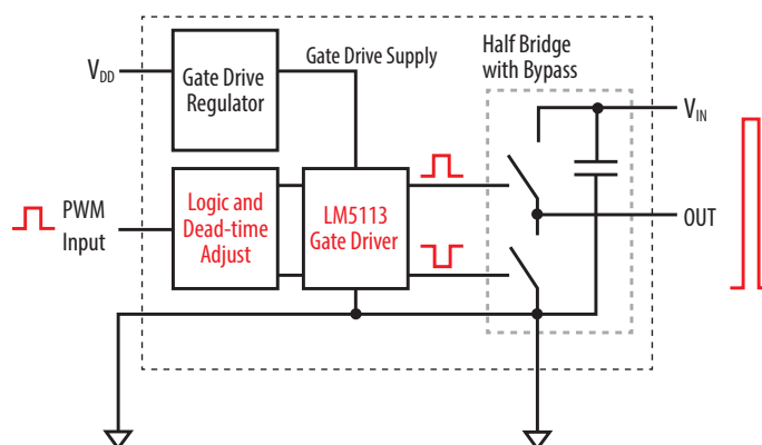
Figure 1: Block Diagram of EPC9057 Development Board
