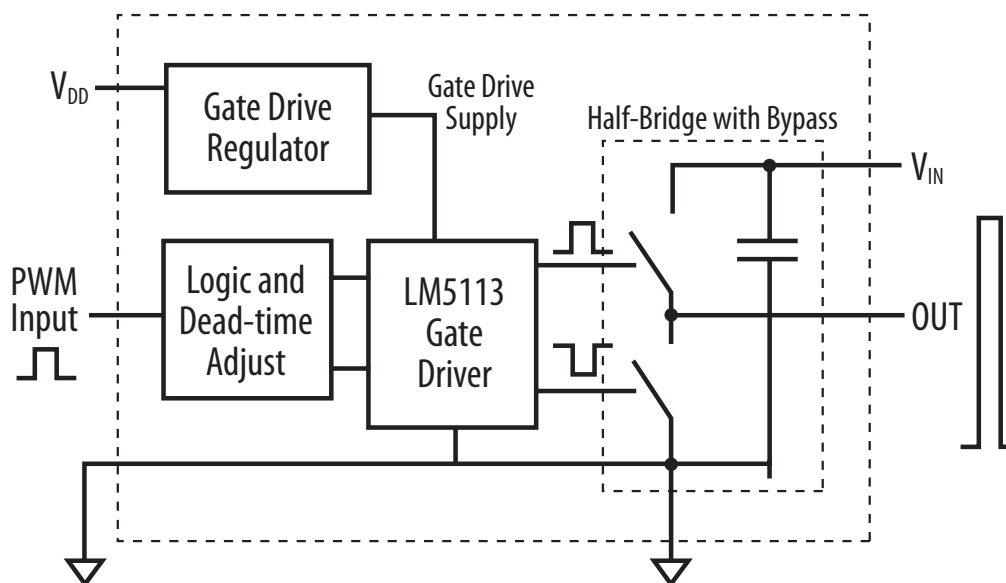
Figure 1: Block Diagram of EPC9005C Development Board
