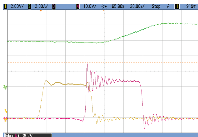
Figure 4: Typical Waveforms for V_{IN} = 24\text{ V} to 1.2\text{ V}/7\text{ A} (1000kHz) Buck converter CH1: V_{pwm} Input voltage – CH2: ( I_{out} ) Switch node current – CH4: ( V_{out} ) Switch node voltage
