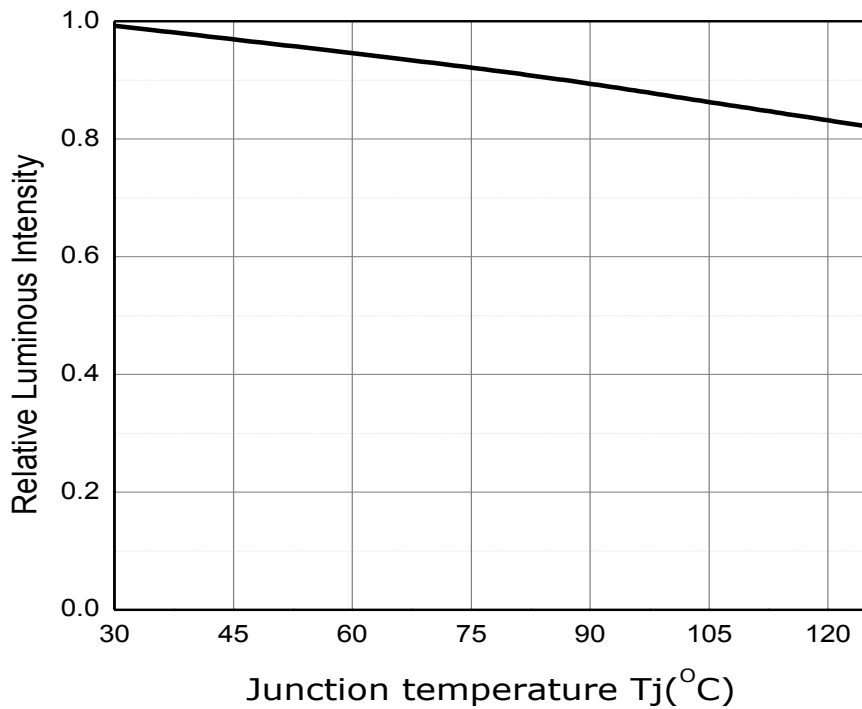
Fig 6. Junction Temperature vs. Relative Luminous Intensity, I_F=100\text{mA}
