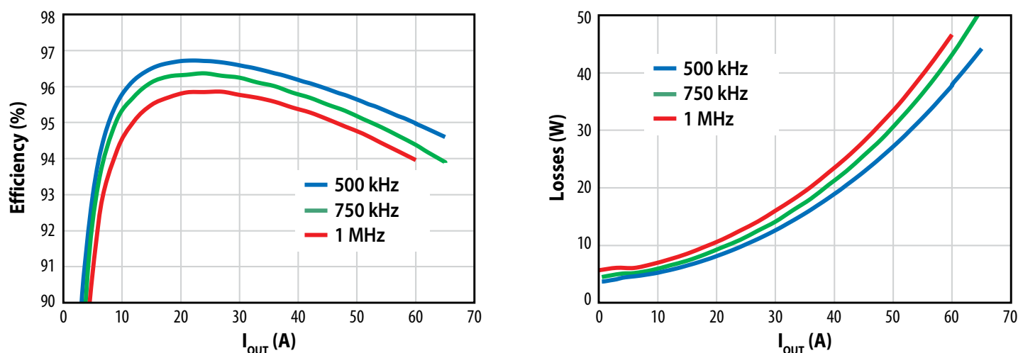
Figure 15: Measured efficiency and power loss operating at at various switching frequencies and using L = 2.2 \mu H
