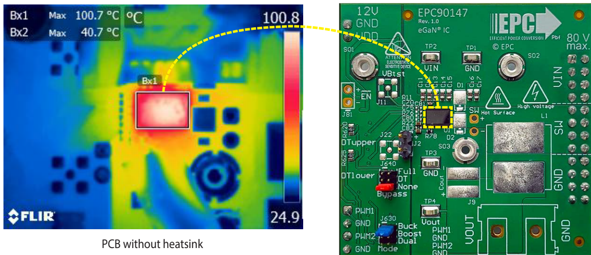
Figure 16: Measured thermal image showing the case temperature when operating under the following conditions: f_s = 500 \text{ kHz} , I_{OUT} = 23 \text{ A} output, 25^{\circ}\text{C} ambient and high airflow
