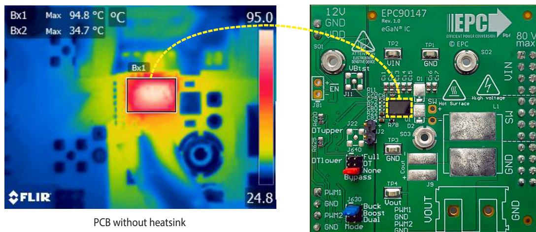
Figure 18: Measured thermal image showing the case temperature when operating under the following conditions: f_s = 1.5 \text{ MHz} , I_{OUT} = 13 \text{ A} output, 25°C ambient and high airflow
