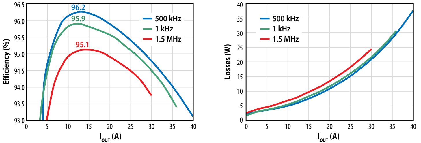
Figure 15: Measured efficiency and power loss operating at various switching frequencies and using L = 2.2 \mu\text{H}
