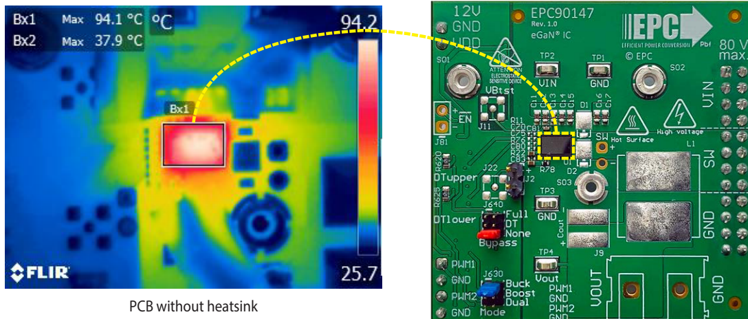
Figure 17: Measured thermal image showing the case temperature when operating under the following conditions: f_s = 1 \text{ MHz} , I_{OUT} = 17 \text{ A} output, 25°C ambient and high airflow
