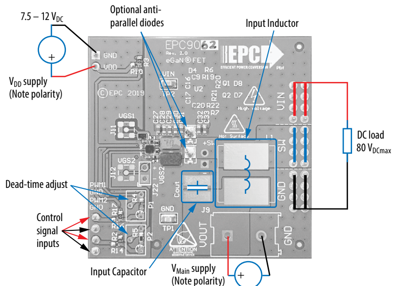
Figure 3: Boost configuration
