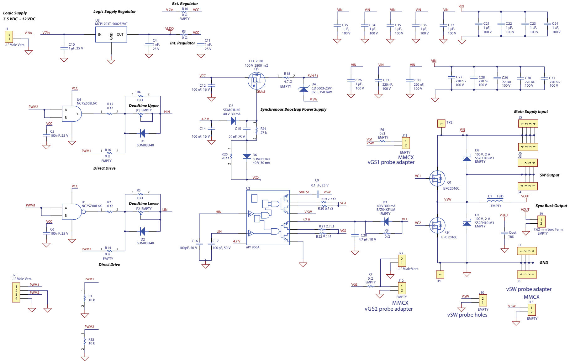
Figure 7: EPC9010C - Schematic
