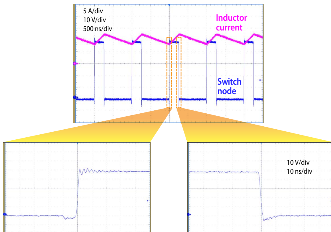
Figure 14: Measured inductor current and switch node waveforms when operating from 48 V at 1 MHz and delivering 10 A into a 12 V load
