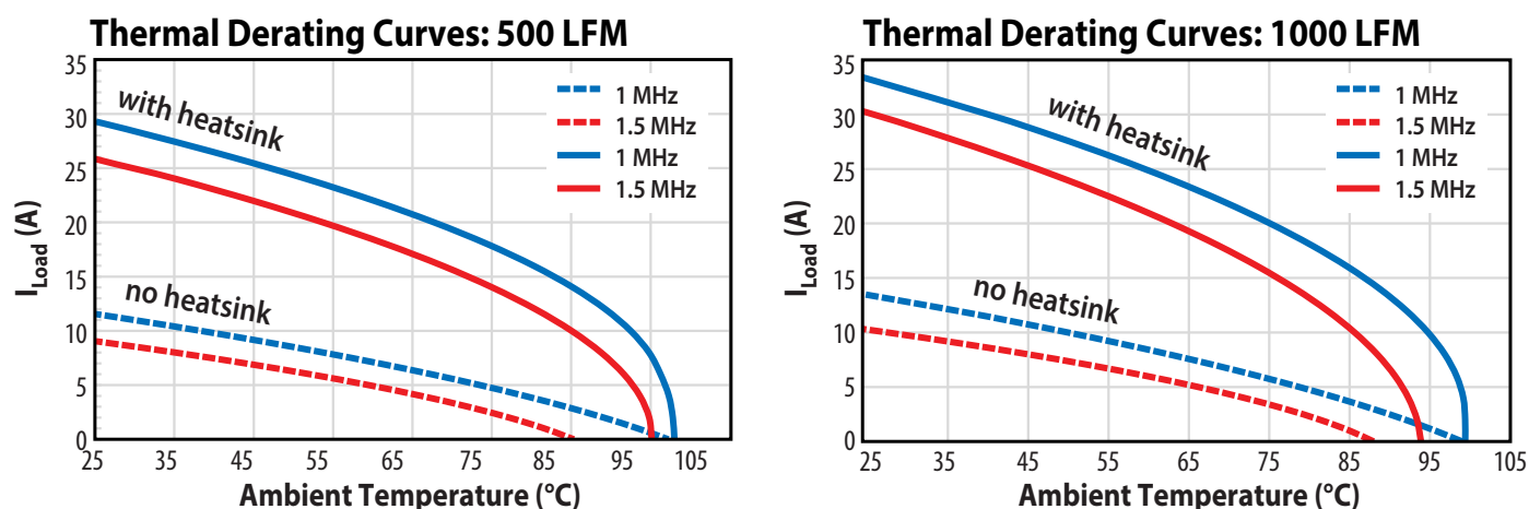
Figure 17: Typical thermal derating curve for two air flow rates, with and without a heatsink attached, measured with the board operating at various switching frequencies and using a 2.2 \mu H inductor
