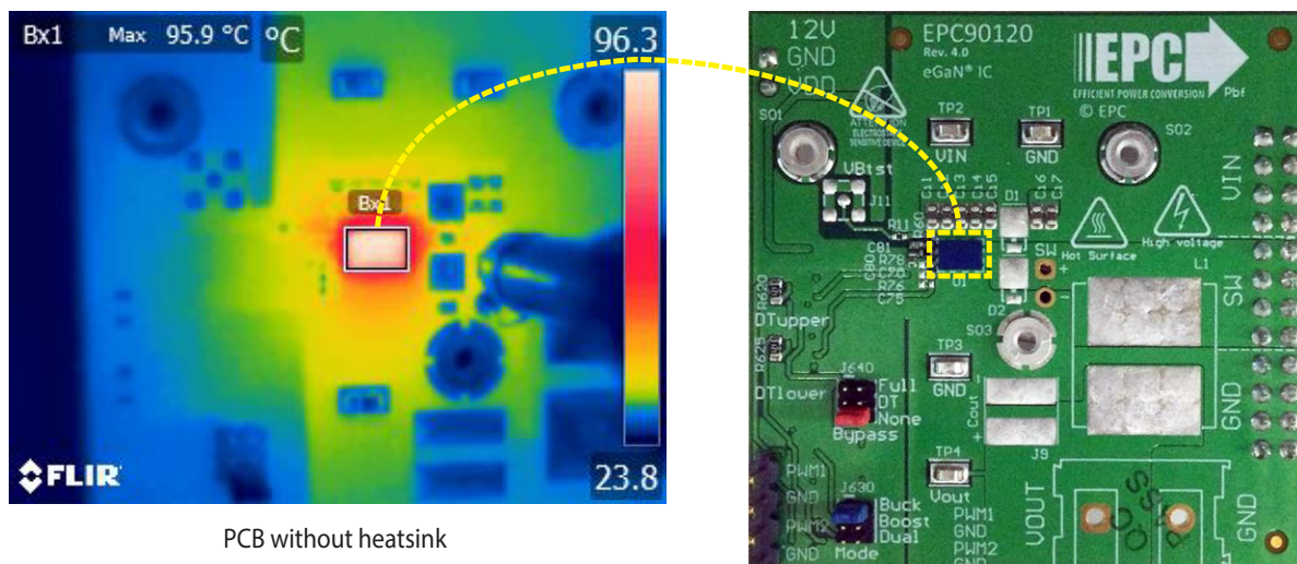
Figure 16: Measured thermal image showing the case temperature when operating under the following conditions: f_s = 1 \text{ MHz} , I_{\text{OUT}} = 10 \text{ A} output, 25°C ambient and high airflow
