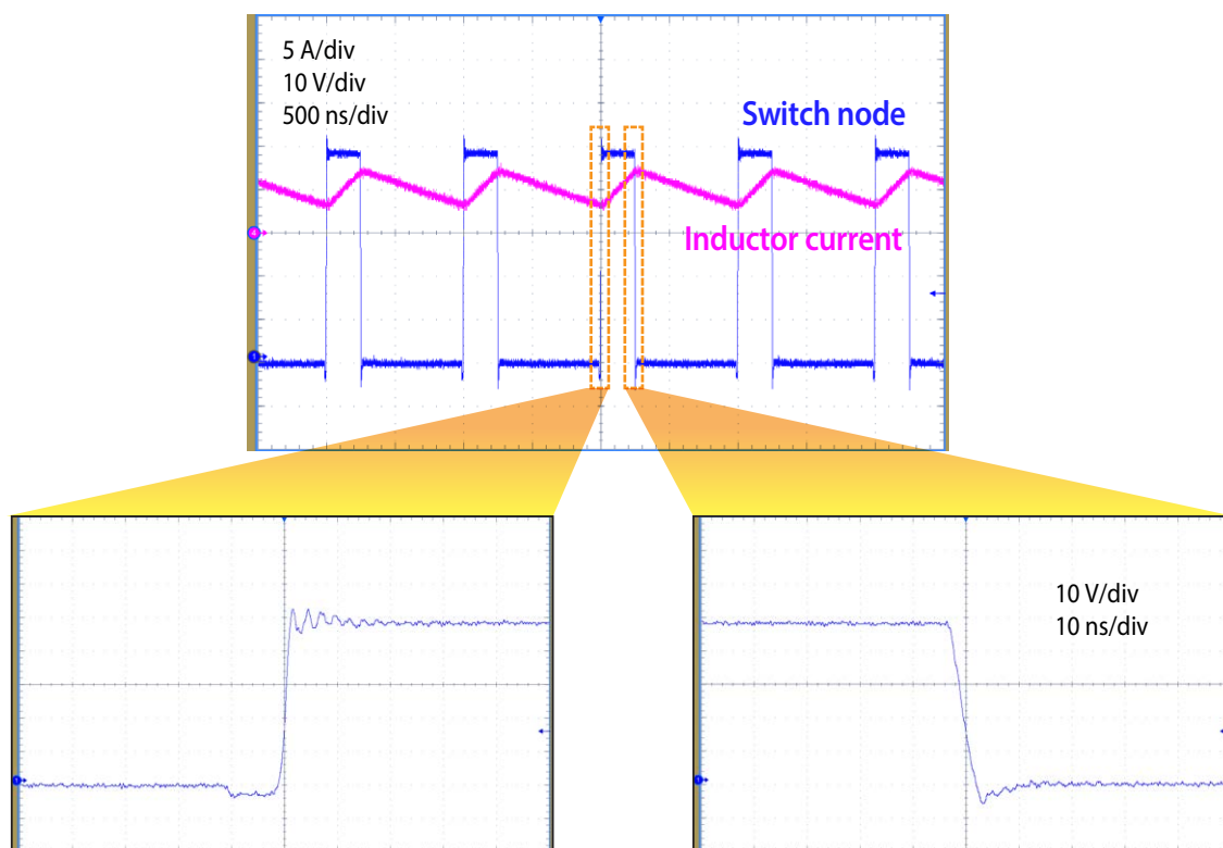
Figure 13: Measured inductor current and switch node waveforms when operating from 48 V at 1 MHz and delivering 5 A into a 12 V load
