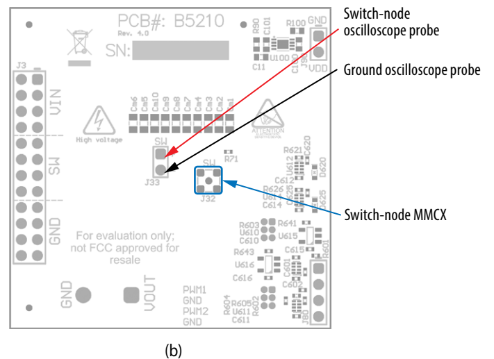
Figure 8: Measurement points (a) front side, (b) Back side
