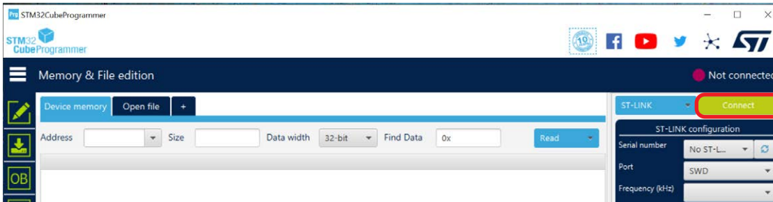
Figure 5: STM32CubeProgrammer
