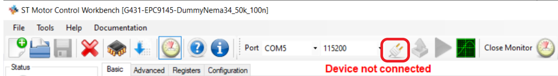
Figure 20: Connect button
