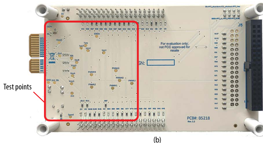
Figure 1: Overview of the EPC9147C board
