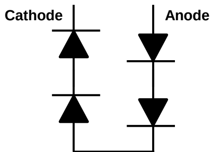
< Inner circuit >
