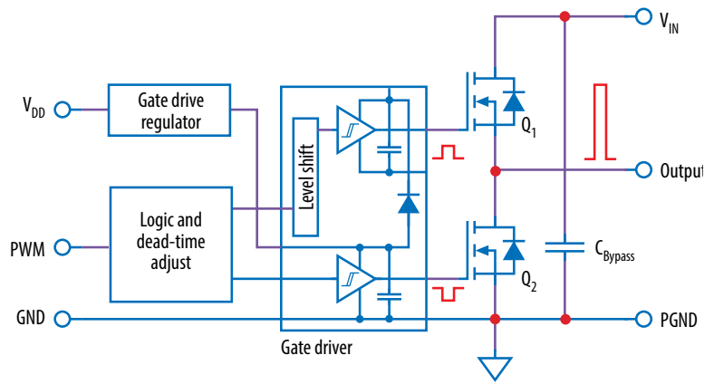
Figure 1: Block diagram of EPC9035 development board
