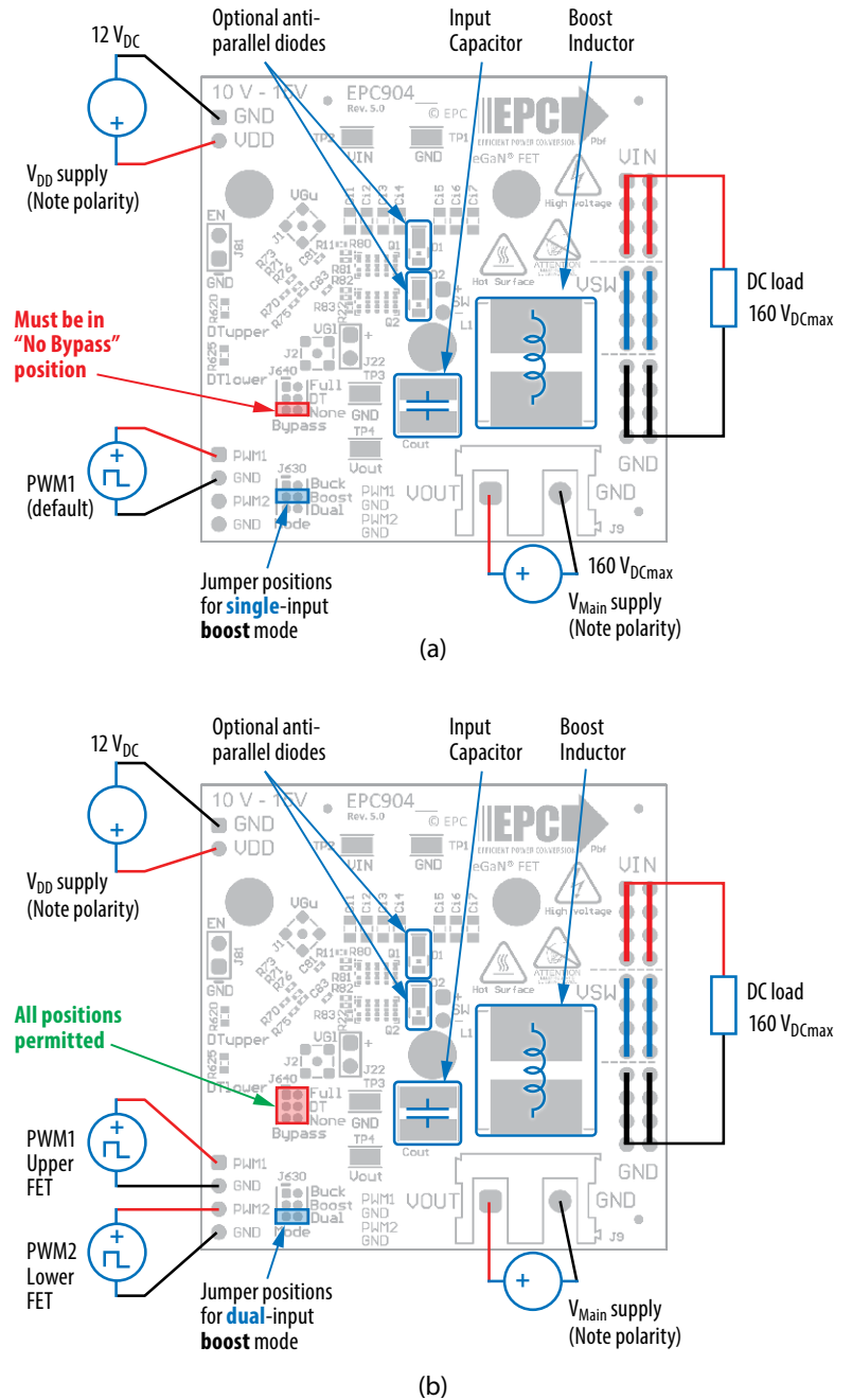
Figure 8: (a) Single-PWM input boost converter (b) Dual-PWM input boost converter configurations showing the supply, inductor, anti-parallel diodes, input capacitor, PWM, and load connections with corresponding jumper settings.
