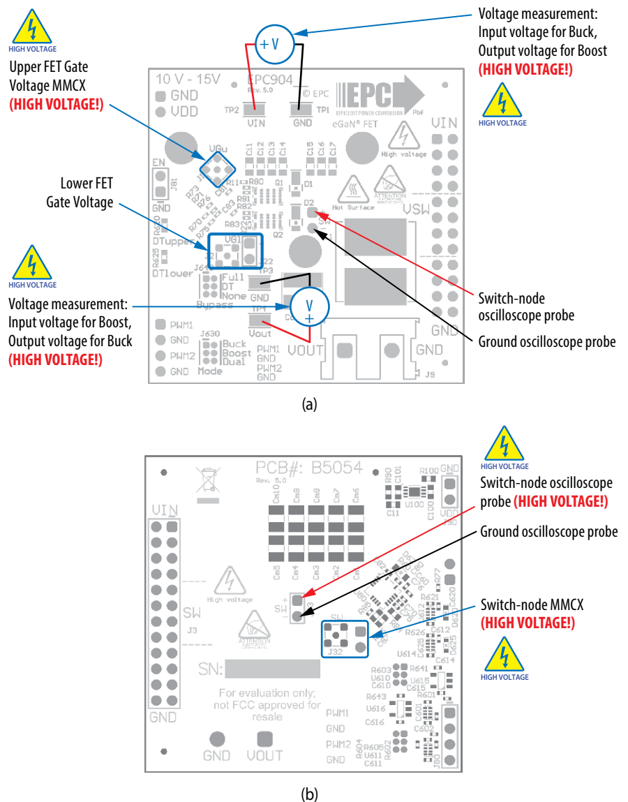
Figure 9: Measurement points (a) front side, (b) Back side
