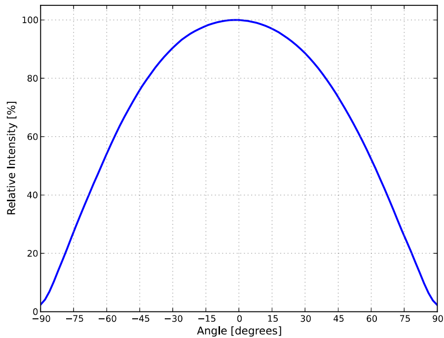
Figure 6. Typical radiation pattern for L1MX-xxxxxxx0 at specified test current, T_j=85^{\circ}\text{C} .
