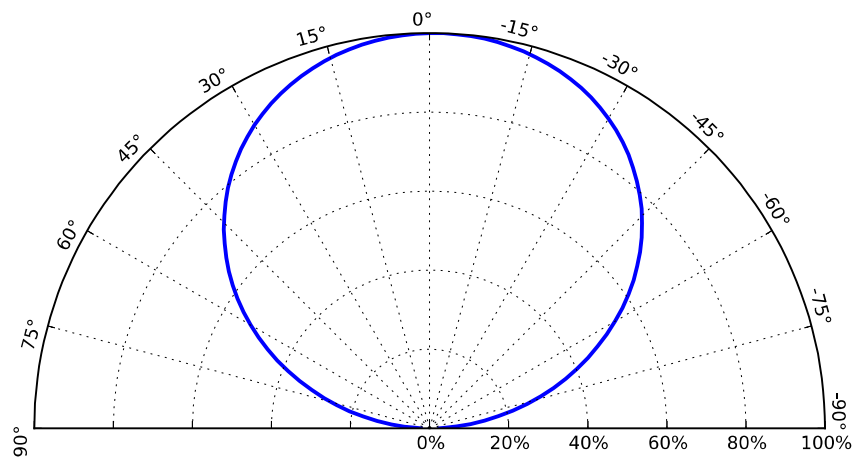
Figure 7. Typical polar radiation pattern for L1MX-xxxxxxx0 at specified test current, T_j=85^{\circ}\text{C} .
