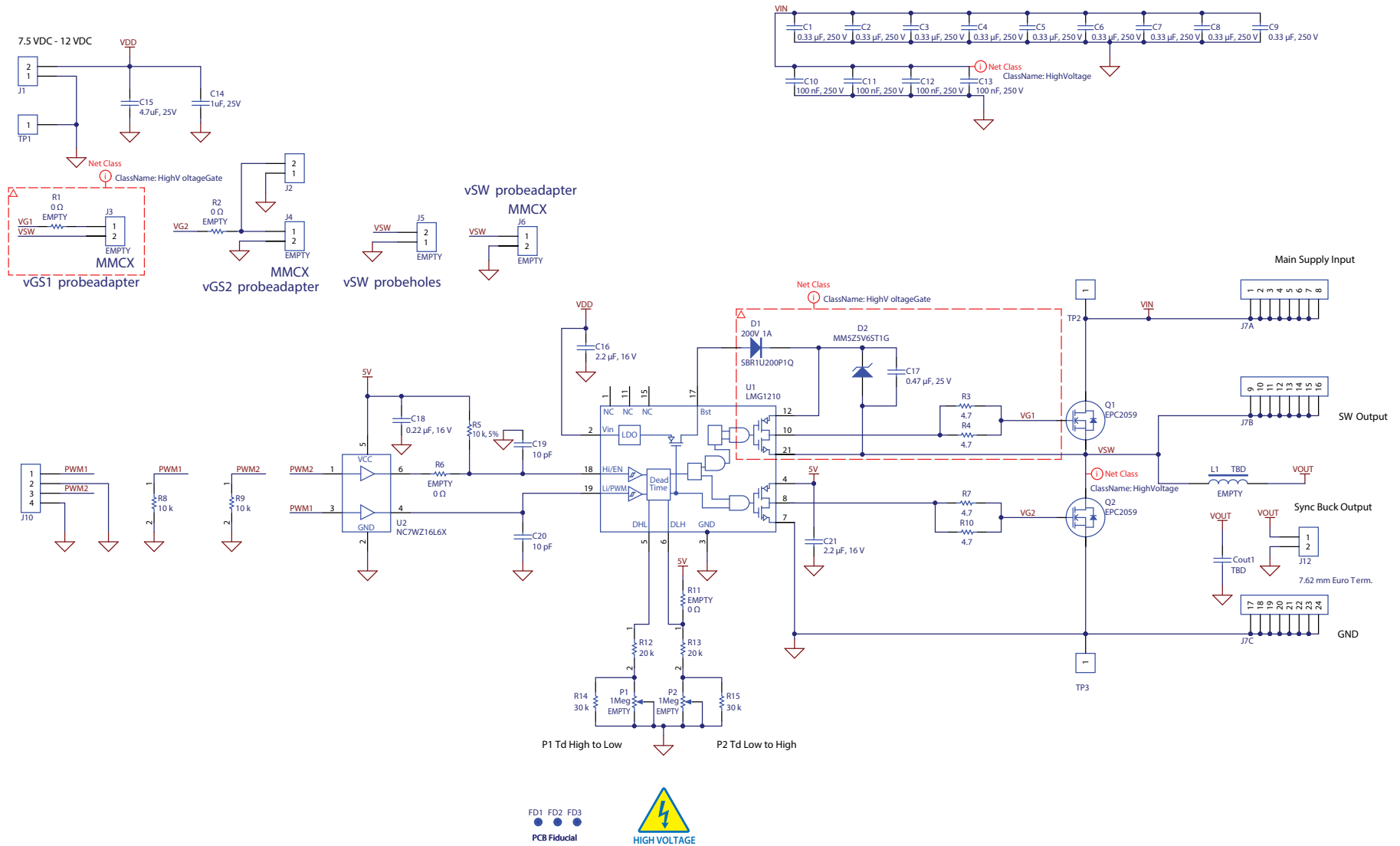
Figure 7: EPC9098 main schematic
