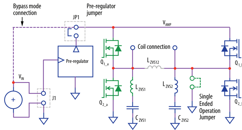
Figure 3: Diagram of EPC9512 ZVS class-D amplifier circuit.
