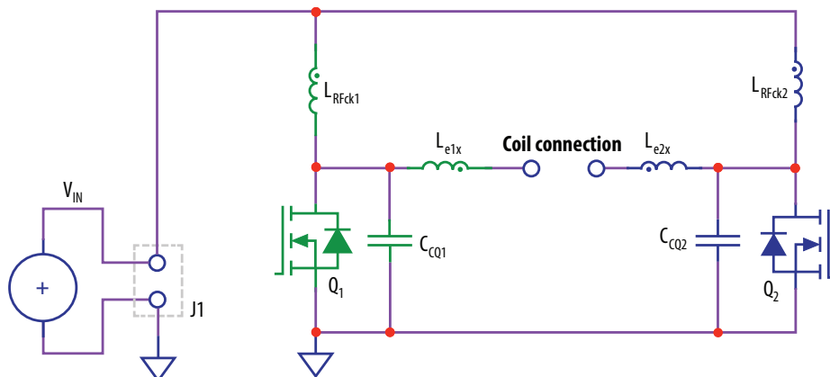
Figure 2: EPC9058 power circuit schematic.
