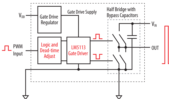
Figure 1: Block Diagram of EPC9059 Development Board
