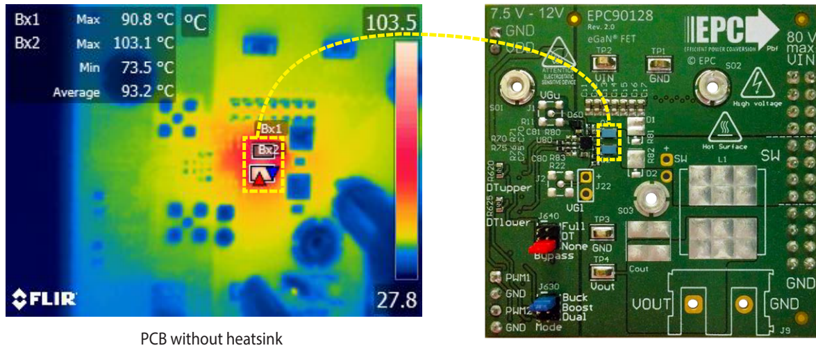
Figure 16: Measured thermal image reading of case temperature when operating under the following conditions: f_s = 500 \text{ kHz} , I_{\text{OUT}} = 14 \text{ A} output, 25^\circ\text{C} ambient and moderate airflow
