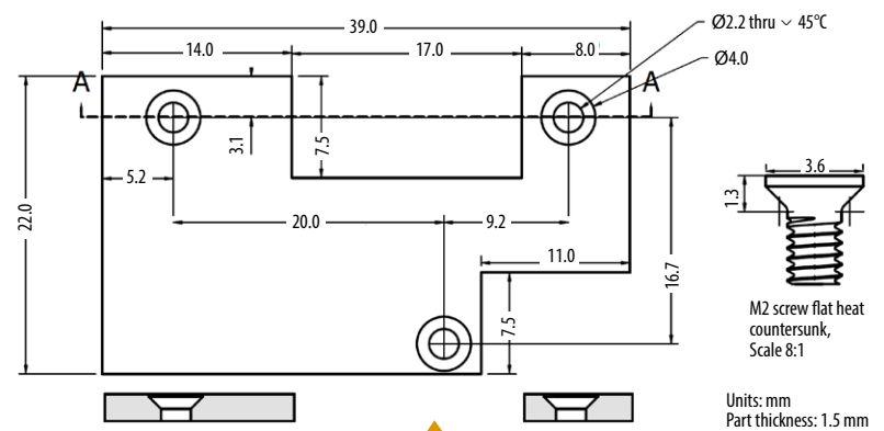
Figure 10: Heat-spreader details
