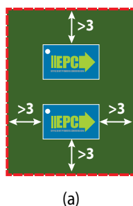
Figure 9: (a) minimum TIM coverage area (b) Insulator sheet details
