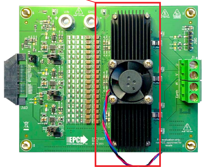
Forced Air Cooling
