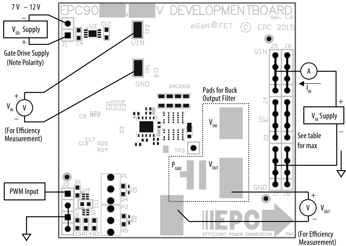
Figure 2: Proper Connection and Measurement Setup
