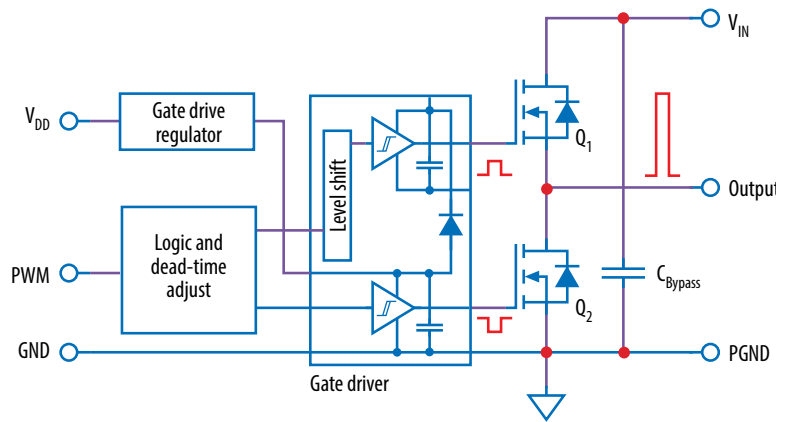
Figure 1: Block diagram of EPC9034 development board
