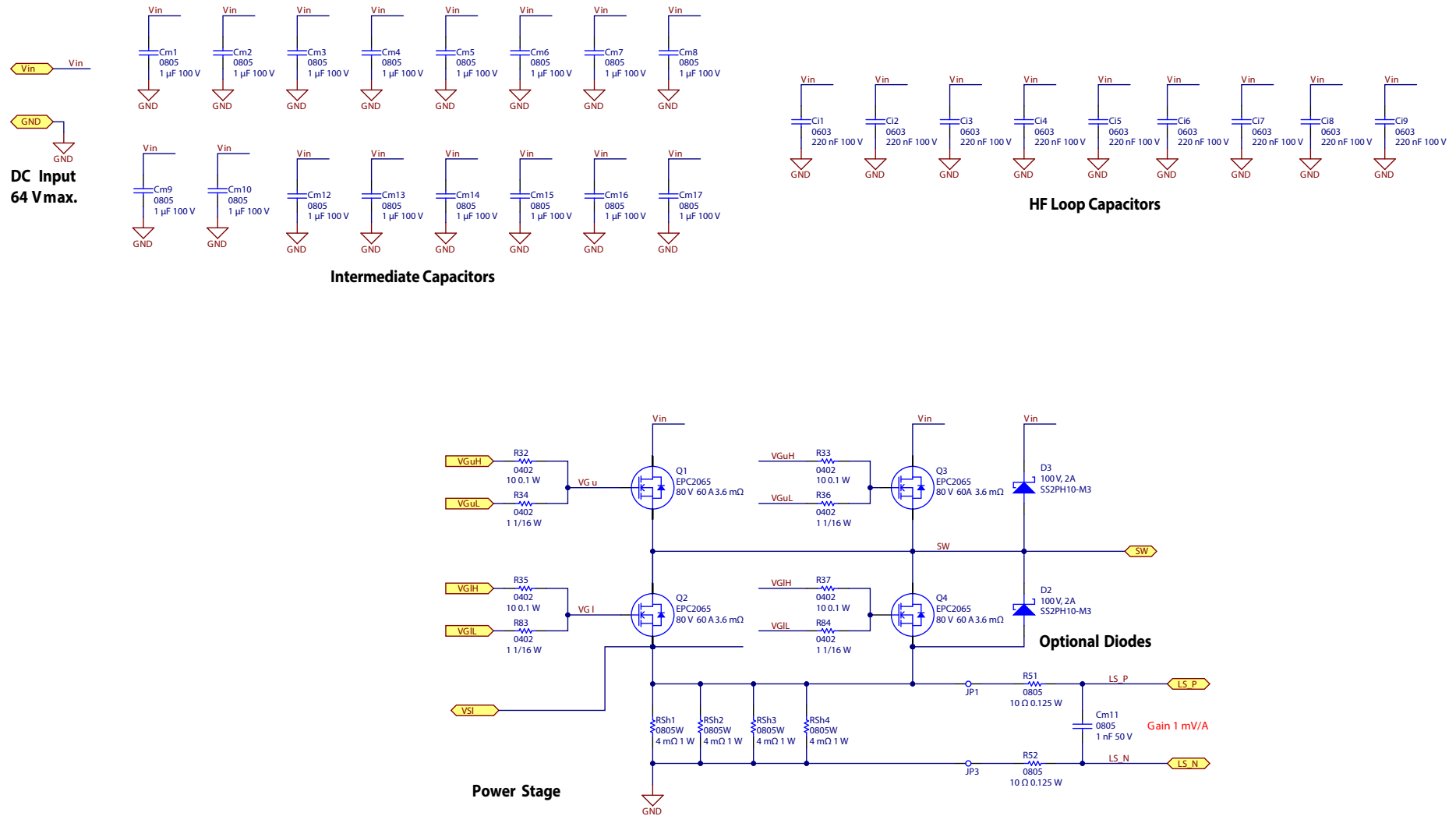
Figure 19: EPC2065 Phase-Leg. In EPC9167 only Q1 and Q2 are mounted. In EPC967HC all four transistors (Q1, Q2, Q3, and Q4) are mounted.
