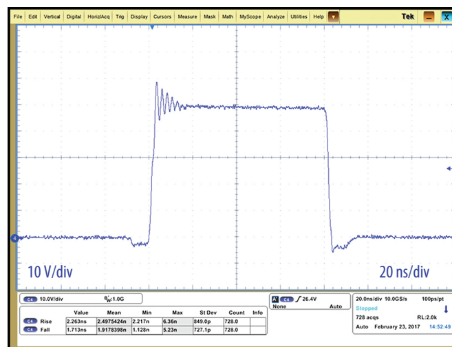
Figure 3: Typical Waveform for V_{IN} = 48 \text{ V} to 1.8 \text{ V}_{OUT} , 10 \text{ A} (500 kHz) Buck Converter
