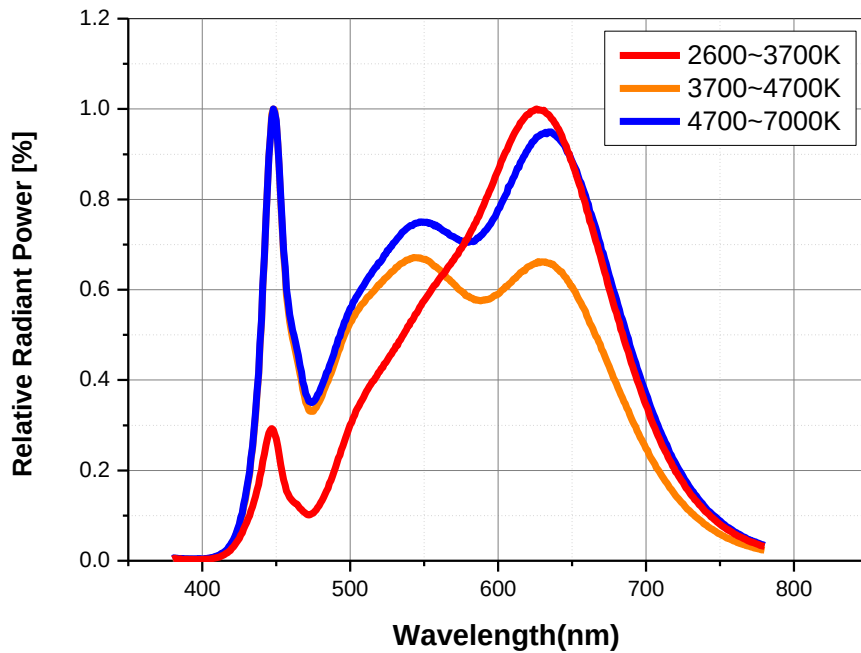
Fig 1. Color Spectrum, T_j = 25^\circ\text{C} , I_F = 20\text{mA}
